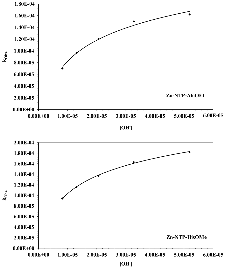
Fig. 3 Plots of k_{\text{obs}} versus [\text{OH}^-] for the hydrolysis of coordinated AlaOEt and HisOMe at 25 °C
